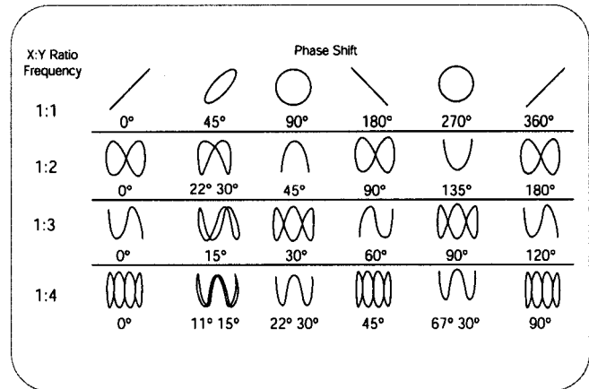
► Figure 70. Lissajous patterns.
