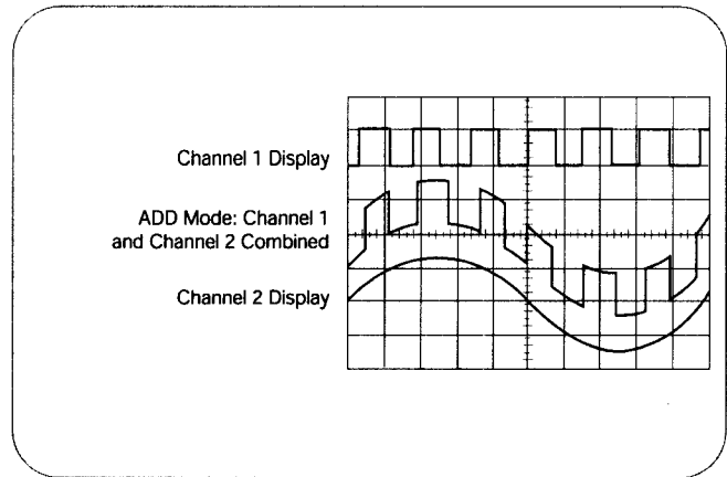
► Figure 39. Adding channels.
