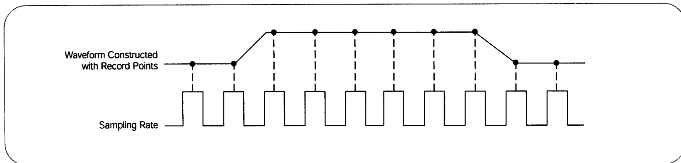
► Figure 29. Real-time sampling method.
