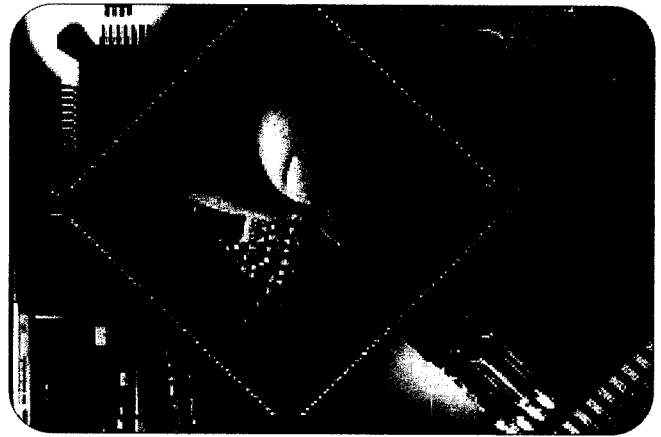
► Figure 45. The Tektronix SF200A and SF500 Series SureFoot™ adapters provide reliable short-lead length probe tip connection to a specific pin on an integrated circuit.
