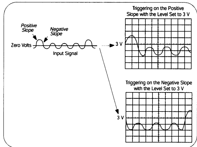
► Figure 36. Positive and negative slope triggering.
