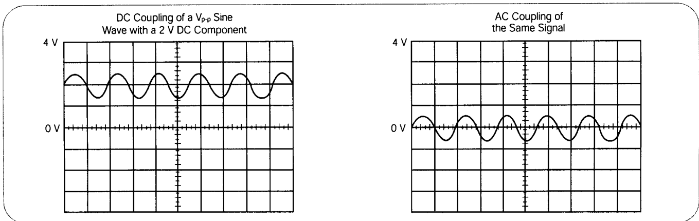
► Figure 23. AC and DC input coupling.
