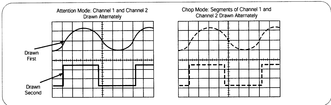
► Figure 24. Multi-channel display modes.
