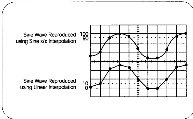
► Figure 31. Linear and sin x/x interpolation.
