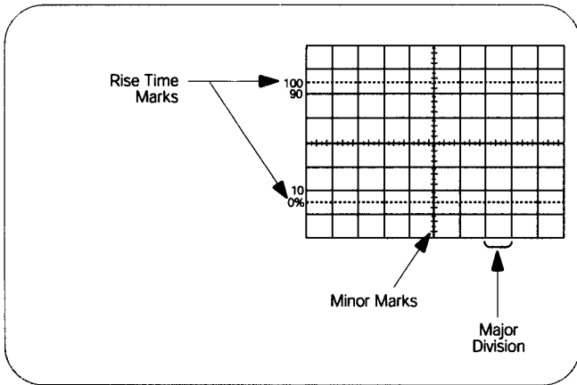
► Figure 38. An oscilloscope graticule.
